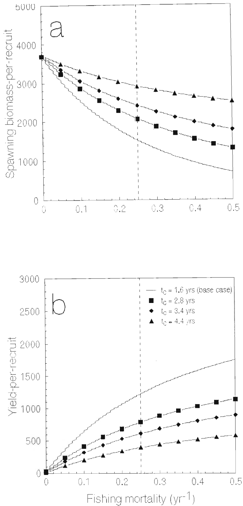
Figure 2 Spawning biomass-per-recruit (a) and yield-per-recruit (b) based on the growth curve SLCA for three different minimum sizes for S. commerson . Dashed line indicates the current fishing mortality.
