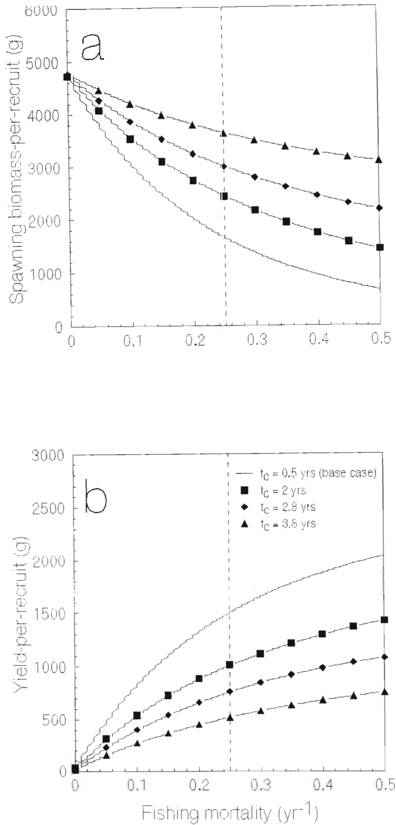
Figure 3 Spawning biomass-per-recruit (a) and yield-per-recruit (b) based on the growth curve VONB 2 for three different minimum sizes for S. commerson . Dashed line shows the current fishing mortality.
