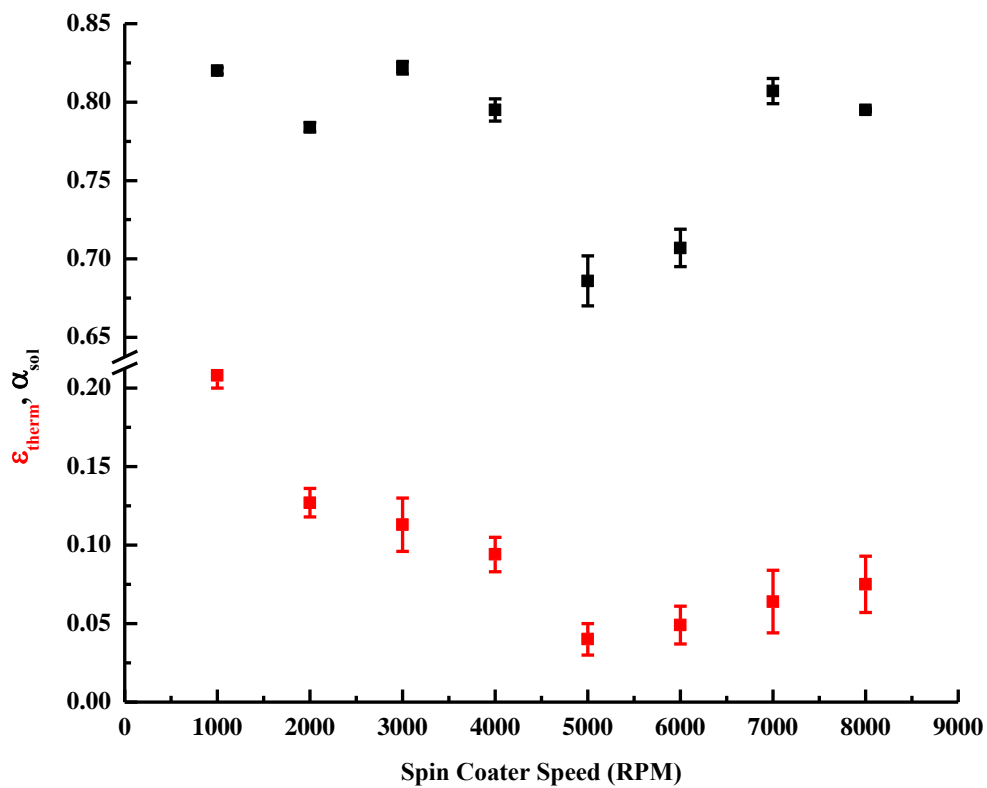
Figure 4.22: \alpha_{\text{sol}} and \epsilon_{\text{therm}} as a function of spin coater speed.
