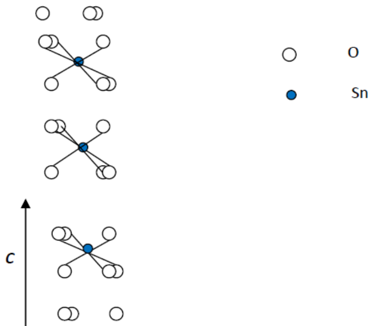
Figure 5.3: Structural model involving the substitution of 4\text{Fe}^{3+} or 4\text{Cr}^{3+} ions by 3\text{Sn}^{4+} ions.
