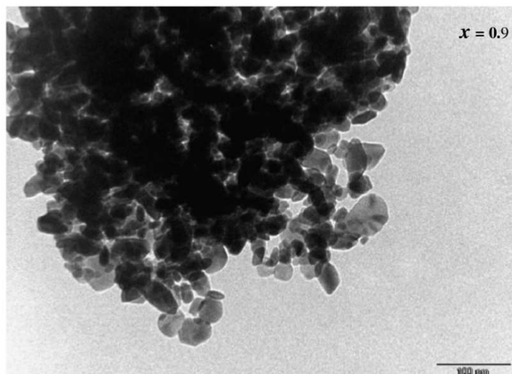
Figure 6.5: TEM micrographs for \text{Mg}_{0.2}\text{Fe}_{0.7}\text{Cr}_{1.1}\text{O}_3 and \text{Mg}_{0.2}\text{Fe}_{0.9}\text{Cr}_{0.9}\text{O}_3 samples.
