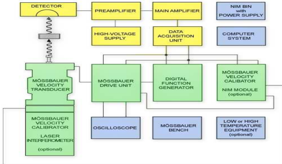
Figure 4.8: Experimental set-up of a Mössbauer spectrometer.
