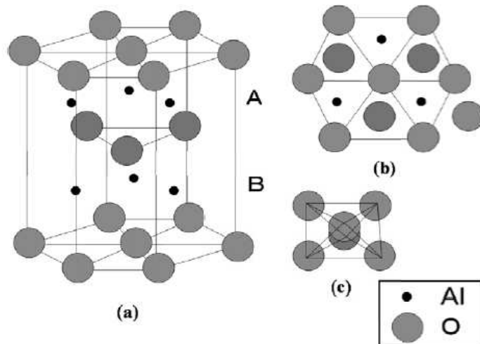
Figure 1.3: (a) Corundum structure in \alpha\text{-Al}_2\text{O}_3 , (b) top view of the corundum structure, and (c) octahedral structure of \alpha\text{-Al}_2\text{O}_3 .
