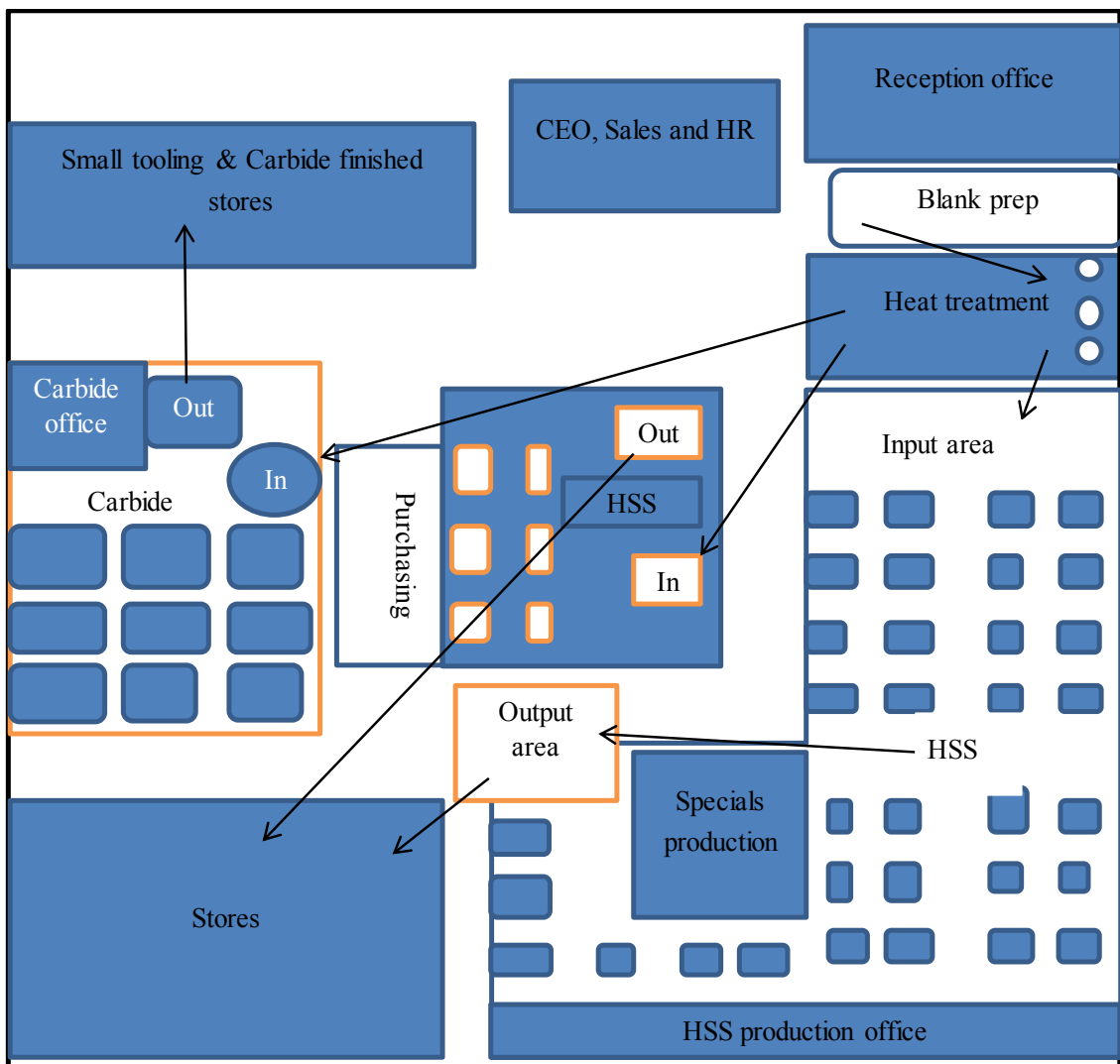
Figure 4.3: Company C layout
