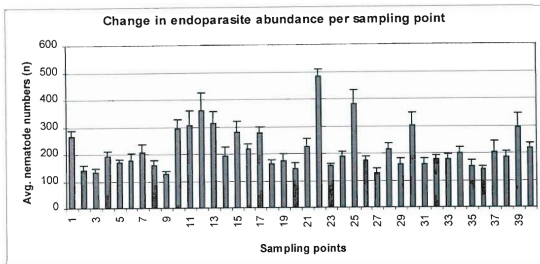
Figure 10: Change in endoparasite abundance in roots at the 40 sampling points along the five transects. Bars represent standard error.
