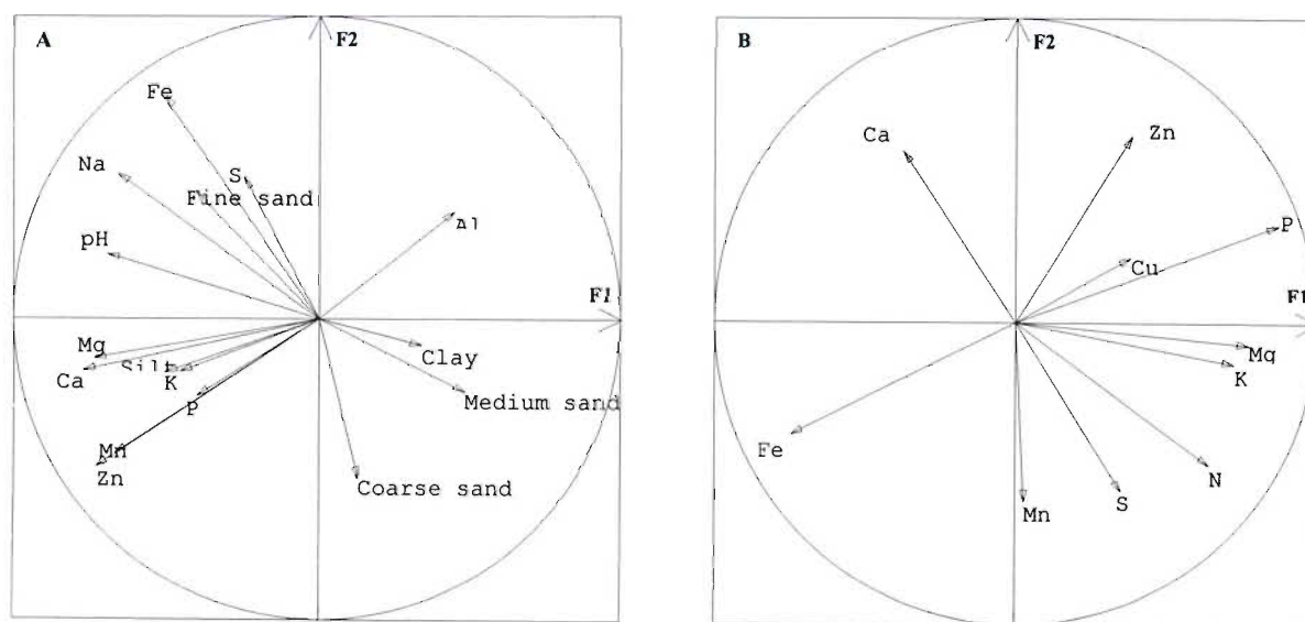
Figure 11: Correlation circles (F1 X F2) of the PCA on soil (A) and leaf element data (B) for the 37 sampling points in Transects 1 and 4.
