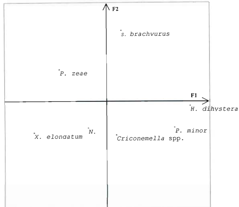
Figure 11: Compromised factorial map (F1 X F2) of the Three-ways Table Analysis on nematode variables for the five transects.
