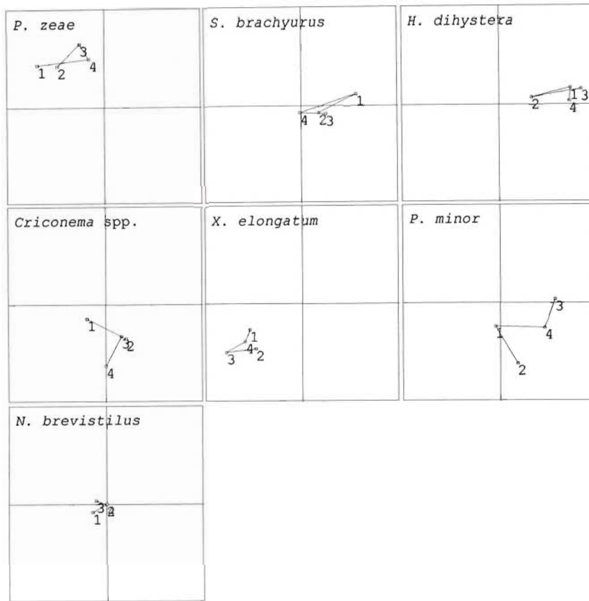
Figure 4: Projection of the four sampling dates for each nematode species on the factorial plan. (1= 1 st date, 2= 2 nd date, 3= 3 rd date, 4 = 4 th date).
