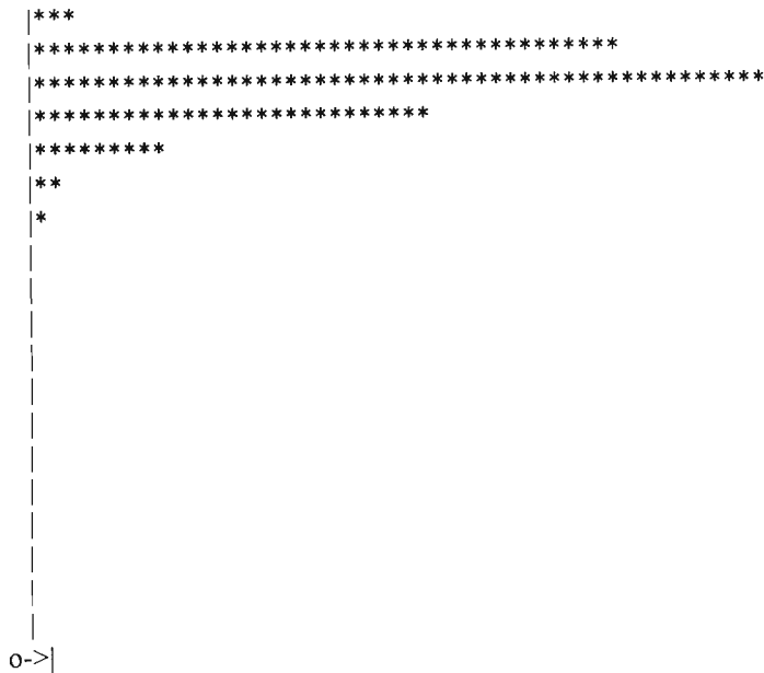
Figure 12: Permutation test of the coinertia analysis for the soil and leaf element data.
