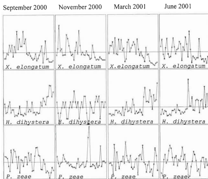
Figure 6: Change of relative percentages of the three important nematode species ( X. elongatum , H. dihystra and P. zaeae ) along the transect on the four sampling dates. The middle line represents the mean in each case.
