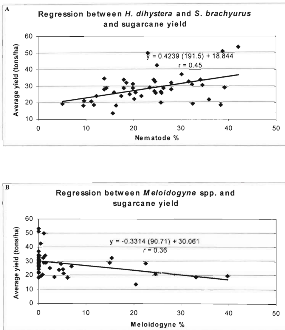
Figure 12: Positive regression between H. dihystra + S. brachyurus and yield (A), and a negative regression between Meloidogyne spp. and yield (B) in the 47 plots.
