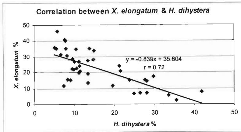
Figure 7: Significant negative regression between X. elongatum and H. dihystra for the four sampling dates (combined).
