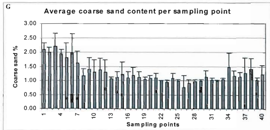
Figure 5: Distribution of magnesium (A) and calcium (B) levels, silt (C), clay (D), medium sand (E), fine sand (F) and coarse sand (G) content at the 40 sampling points along the five transects. Bars represent standard errors.
