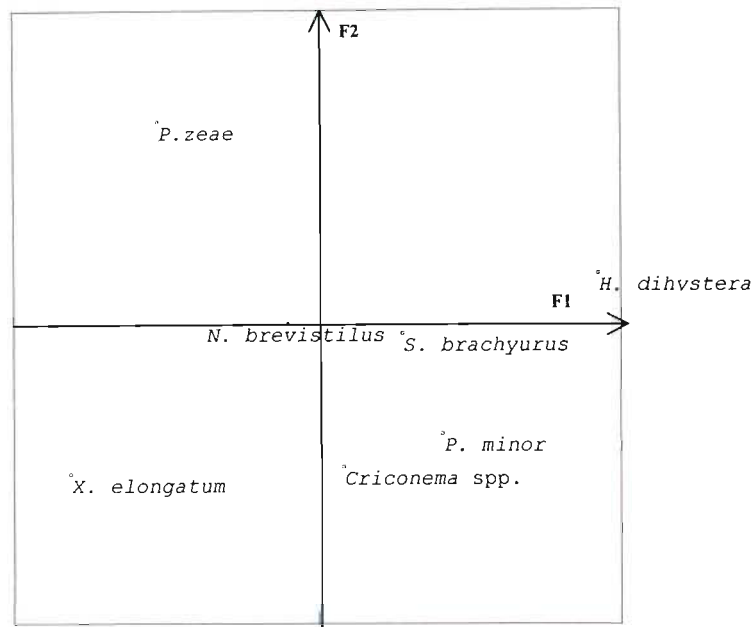
Figure 3: Compromised factorial map (F1 X F2) of the Three-ways Table Analysis on nematode variables for the four sampling dates. F1 = first factor, F2 = second factor.
