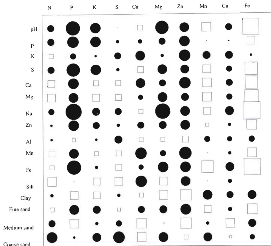
Figure 13: Crossed coinertia table showing the relationship between soil and leaf elements. Circles represent a positive correlation while squares represent a negative correlation. The size of the symbol is proportional to the absolute value.
