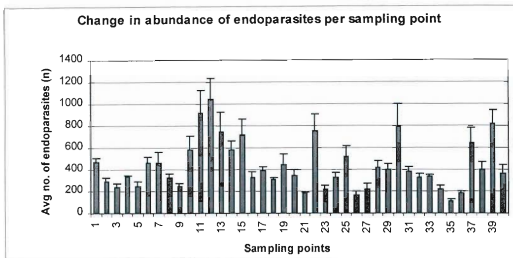
Figure 2: Change in endoparasite abundance in roots per sampling point for the four dates.
