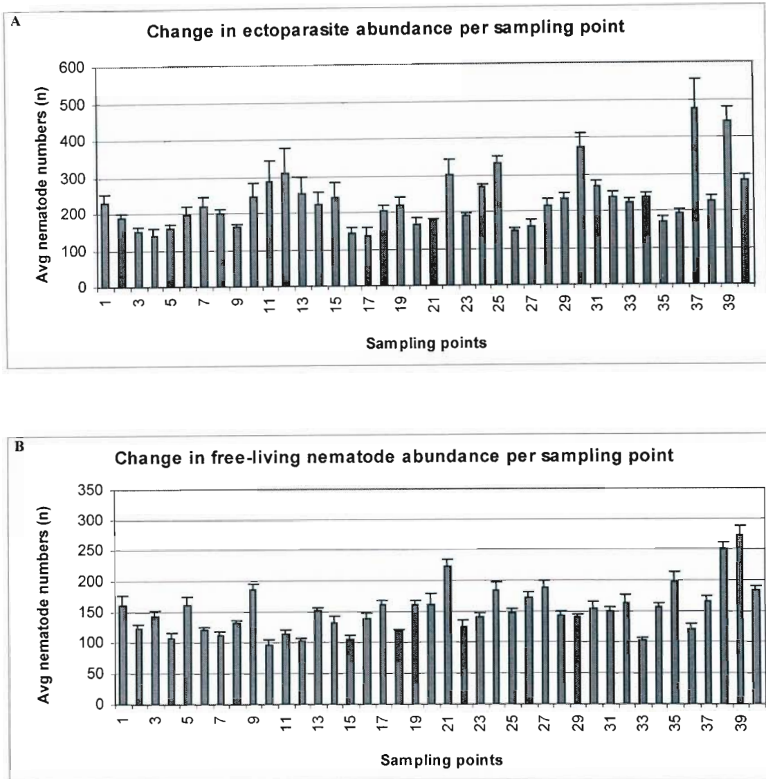
Figure 9: Change in nematode distribution in soil at the 40 sampling points along the five transects, (A) ectoparasites in soil, (B) free-living nematodes in soil. Bars represent standard error.
