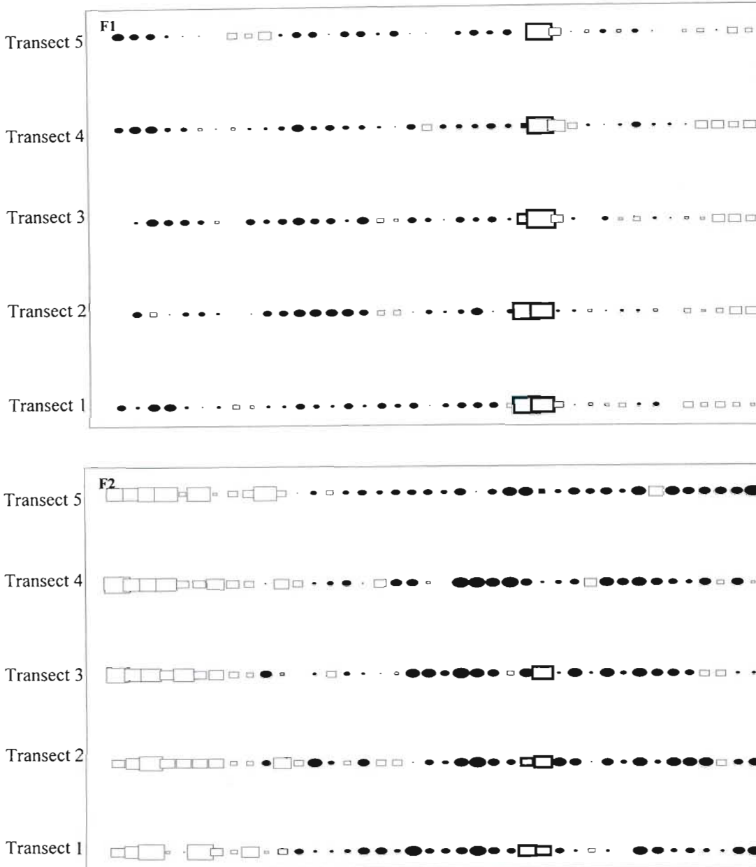
Figure 2: First and second factorial values of the PCA on the values of soil elements and soil particles for the 40 sampling points projected on the trial map. Circles correspond to positive factorial values and squares correspond to negative factorial values. The size of the symbol is proportional to the absolute value.
