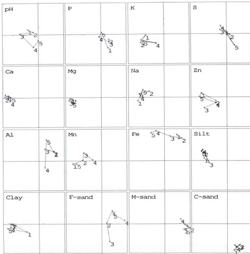
Figure 4: Projection of the five transects per soil elements and particles on the factorial plan (1 = transect 1, 2 = transect 2, 3 = transect 3, 4 = transect 4, 5 = transect 5).
