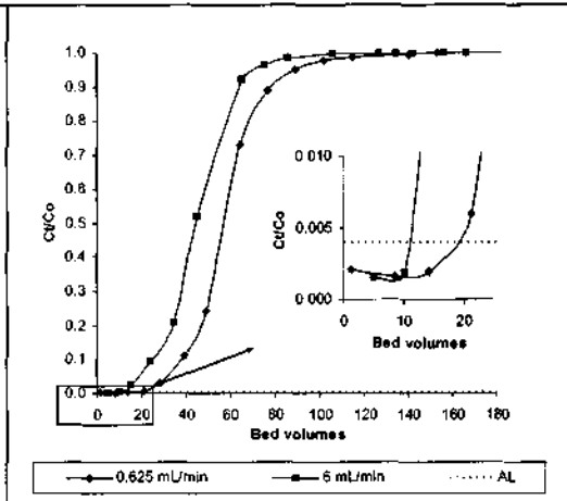
Fig 5.7 : Black breakthrough curve at different flowrates and 60°C
