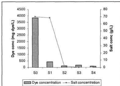
Fig 3.1: Dye and salt concentrations before and after dyeing of Navy shade. S0 -unexhausted dyebath, S1 -exhausted dyebath, S2 -cold water rinse, S3 -hot soaping and S4 -cold water rinse.
