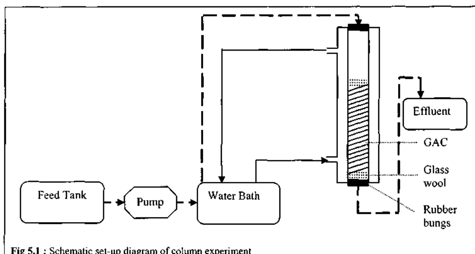
Fig 5.1 : Schematic set-up diagram of column experiment
