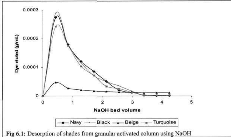
Fig 6.1: Desorption of shades from granular activated column using NaOH
