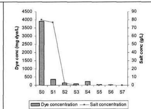
Fig 3.2: Dye and salt concentrations before and after dyeing of Black shade. S0 -unexhausted dyebath, S1 -exhausted dyebath, S2 -warm water rinse, S3 -cold neutralisation, S4 -hot soaping and S5 -hot water rinse, S6 -warm water rinse and S7 -cold water rinse.
