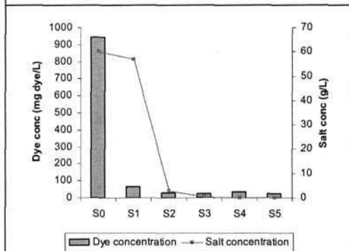
Fig 3.3: Dye and salt concentrations before and after dyeing of Beige shade. S0 -unexhausted dyebath, S1 -exhausted dyebath, S2 -hot water rinse, S3 -cold water rinse, S4 -hot soaping and S5 -cold water rinse.
