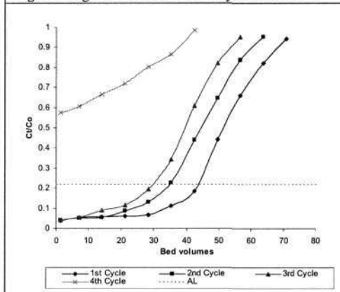
Fig 6.4: Regeneration of GAC-Beige shade at 60°C AL-Acceptable Limit for reuse
