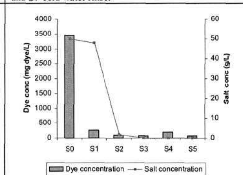
Fig 3.4: Dye and salt concentrations before and after dyeing of Turquoise shade. S0 -unexhausted dyebath, S1 -exhausted dyebath, S2 -cold water rinse, S3 -cold neutralisation, S4 -hot soaping and S5 -cold water rinse.
