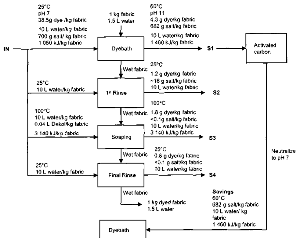
Fig 4.21: Flow diagram and mass balance for dyeing of Navy shade
