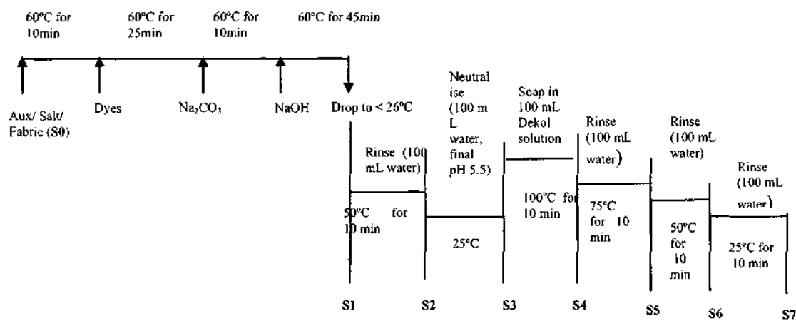
Fig A.2: Black shade dyeing process
