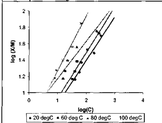
Fig 4.11 : Effect of temperature on adsorption of Beige shade at pH 11 and 60 g/L NaCl
