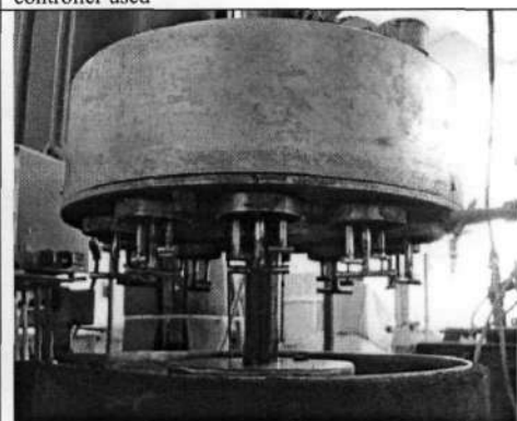
Fig 4.4 : Stirrers view where metal flasks are clamped
