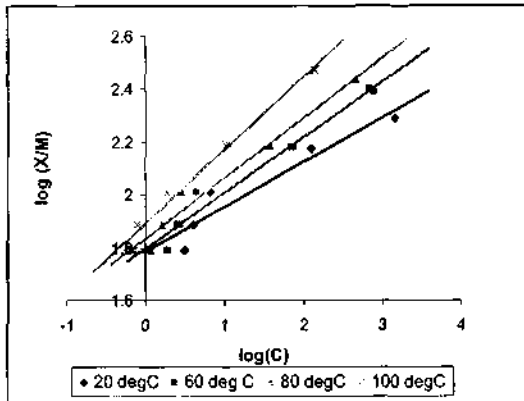
Fig 4.9 : Effect of temperature on adsorption of Navy shade at pH 11 and 70 g/L NaCl
