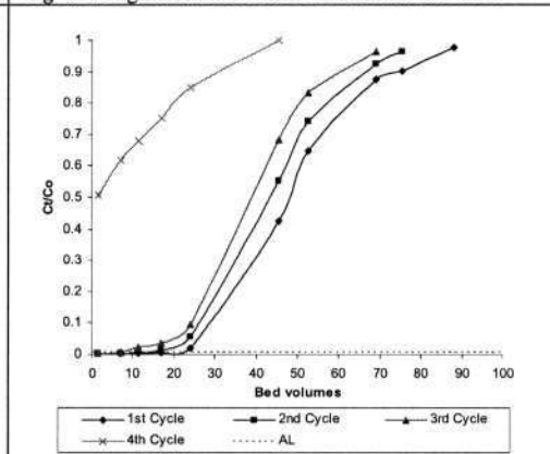
Fig 6.5: Regeneration of GAC-Turquoise shade at 60°C
