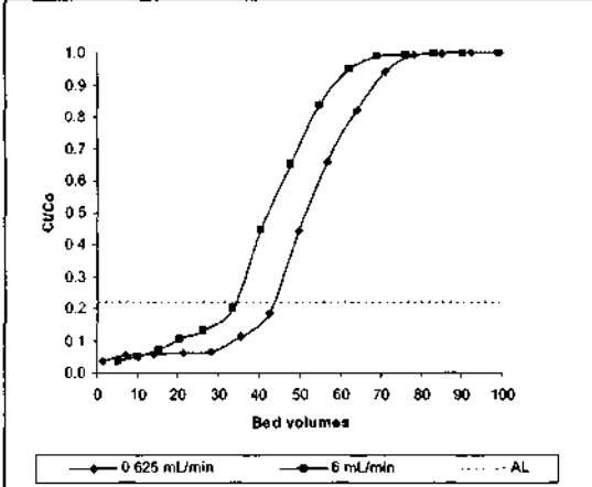
Fig 5.8 : Beige breakthrough curve at different flowrates and 60°C
