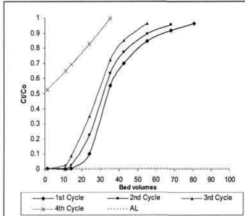
Fig 6.2: Regeneration of GAC-Navy shade at 60°C
