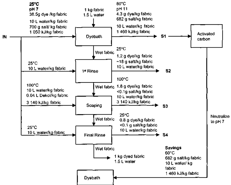
Fig B.1: Flow diagram and mass balance for dyeing of Navy shade with recovery
