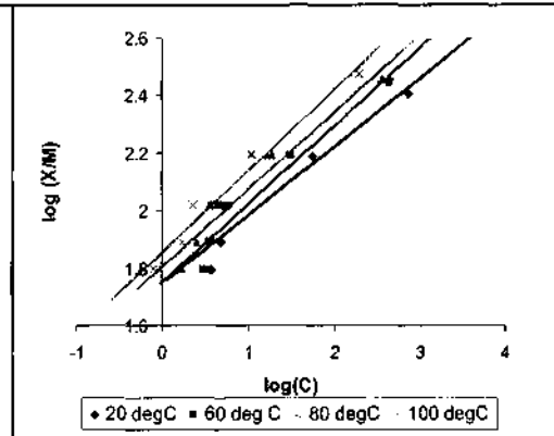
Fig 4.10 : Effect of temperature on adsorption of Black shade at pH 11 and 80 g/L Na 2 SO 4
