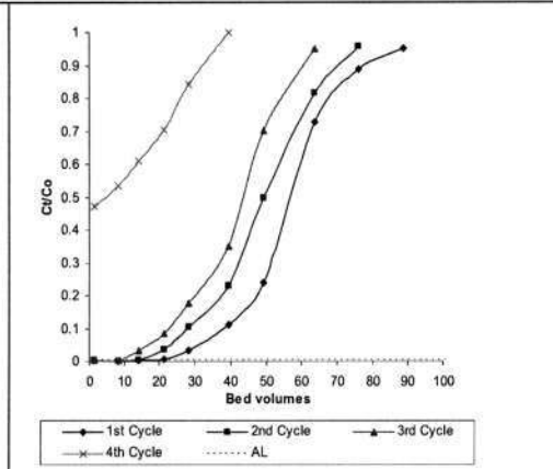
Fig 6.3: Regeneration of GAC-Black shade at 60°C
