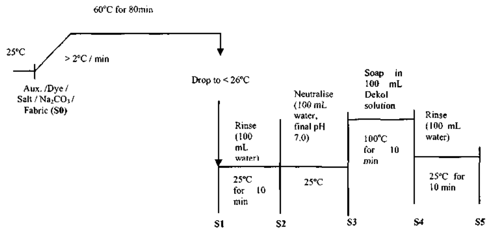
Fig A.4: Turquoise shade dyeing process
