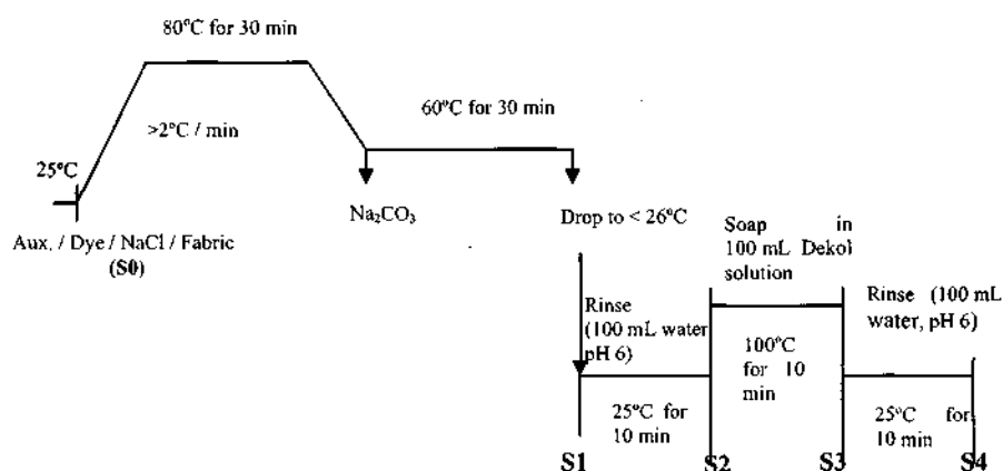
Fig A.1: Navy shade dyeing process
