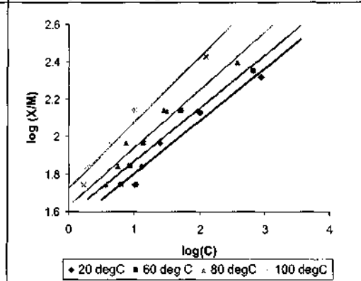
Fig 4.12 : Effect of temperature on adsorption of Turquoise shade at pH 10 and 50 g/L Na 2 SO 4
